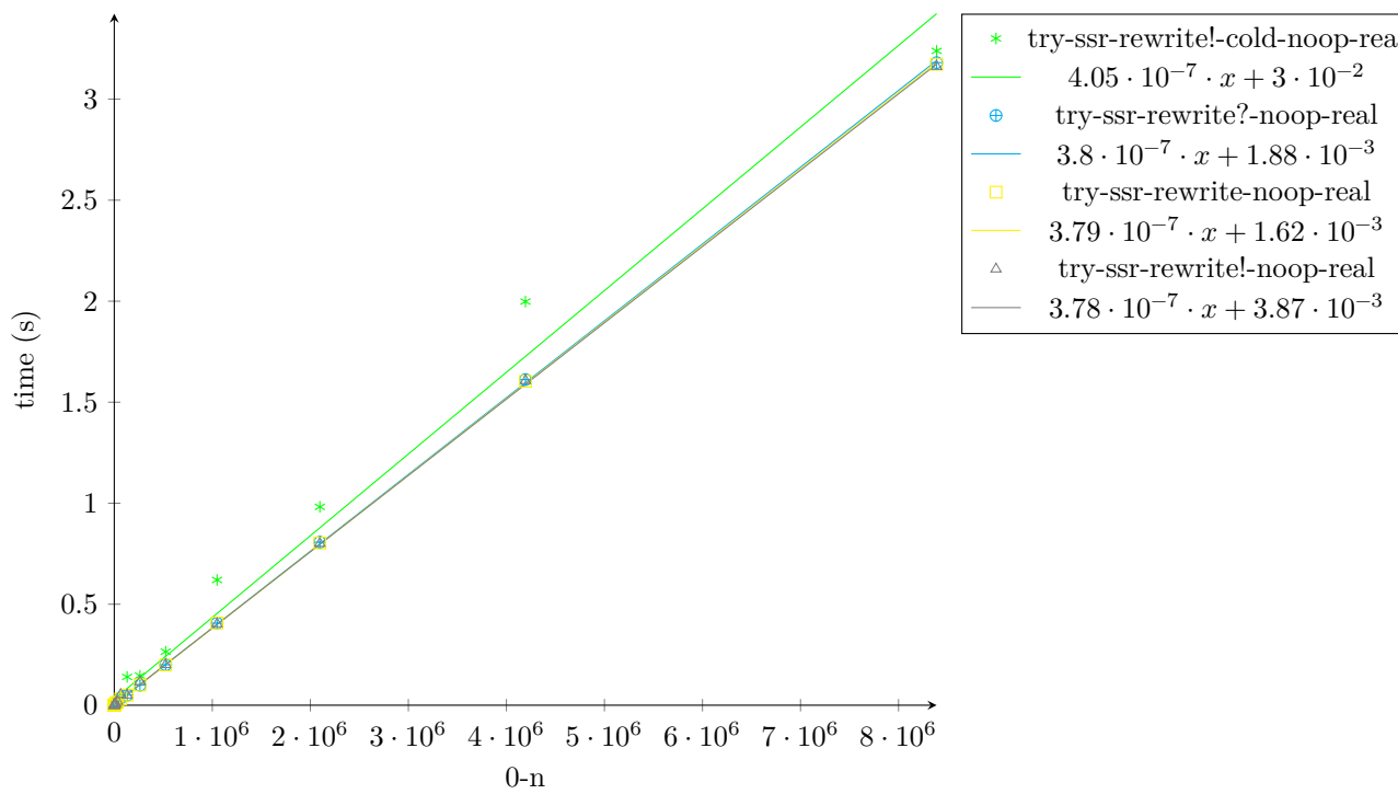
Figure 24: timing-rewrite-repeated-app-ssrrewrite-noop param-1-lgn 1
