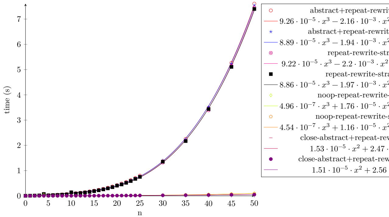
Figure 18: timing-rewrite-strat-under-binders
