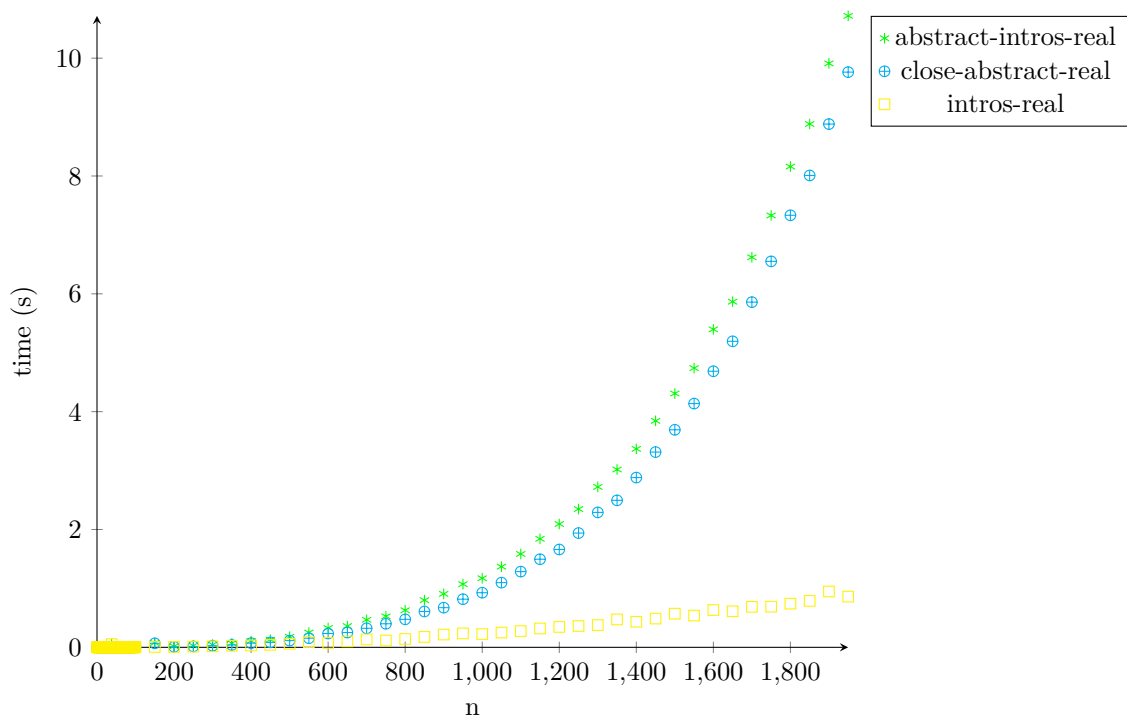
Figure 15: timing-intros-n-fun
