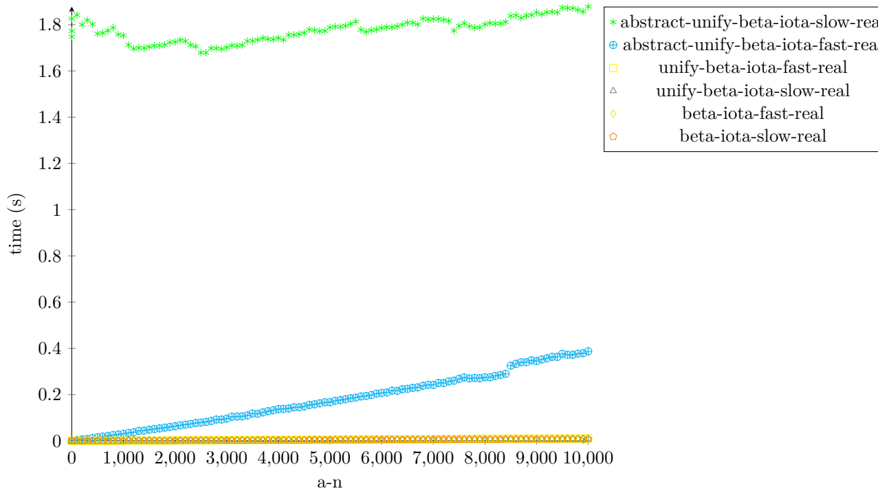
Figure 41: timing-iota-reduction-with-abstract-fact9 param-fact-n 9
