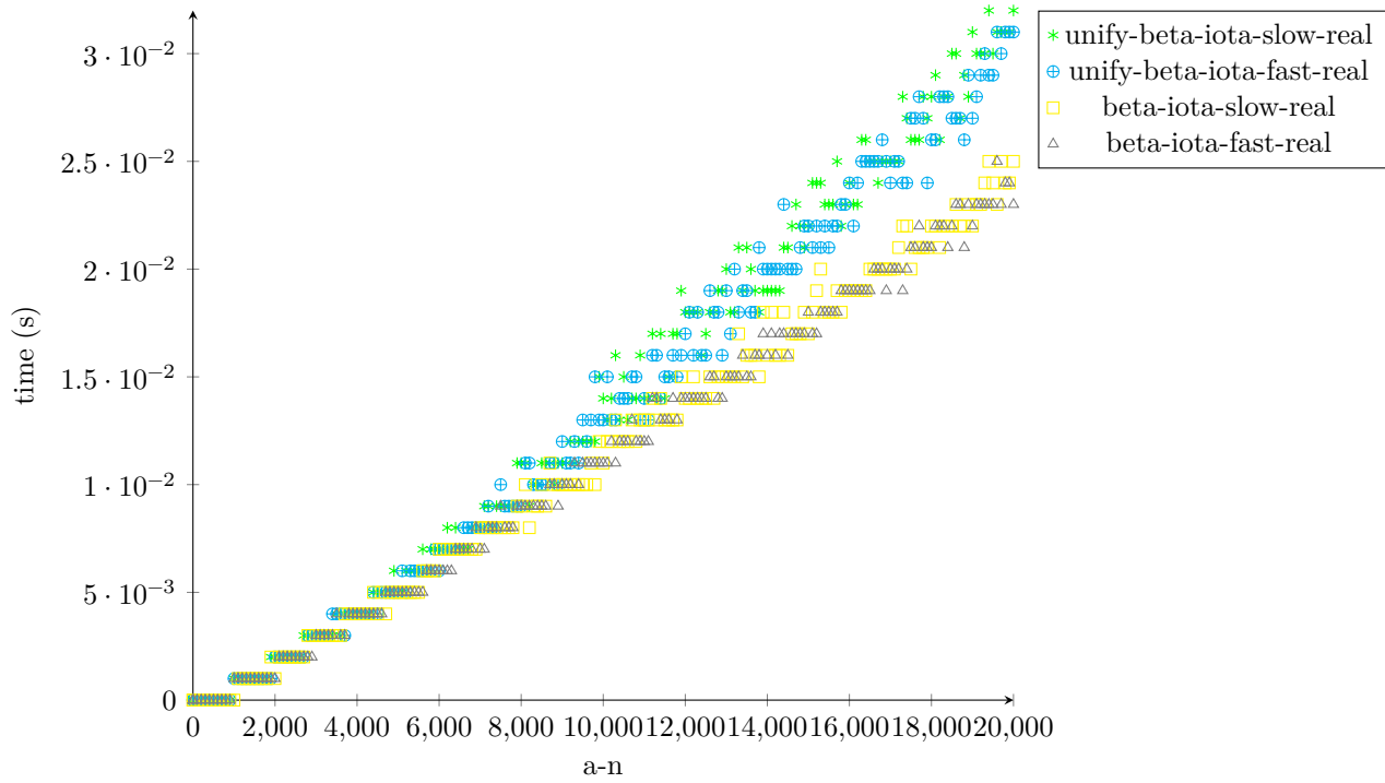
Figure 39: timing-iota-reduction-fact9 param-fact-n 9
