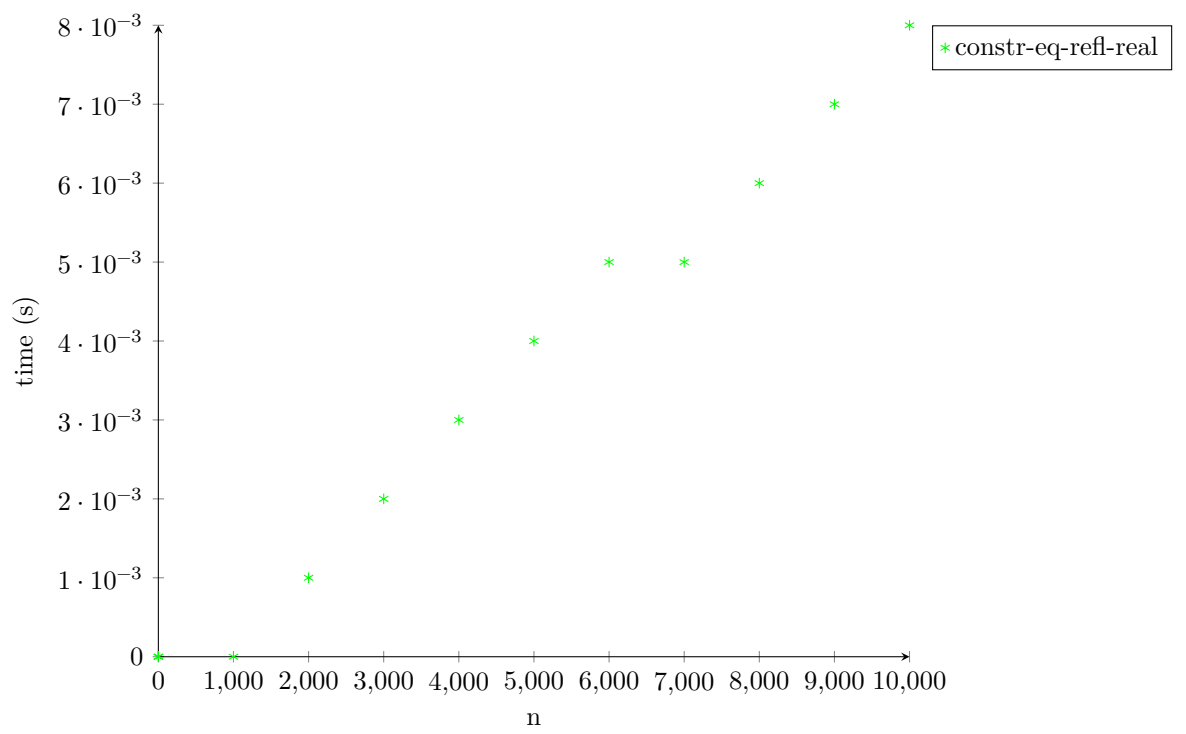
Figure 29: timing-constr-eq-alpha
