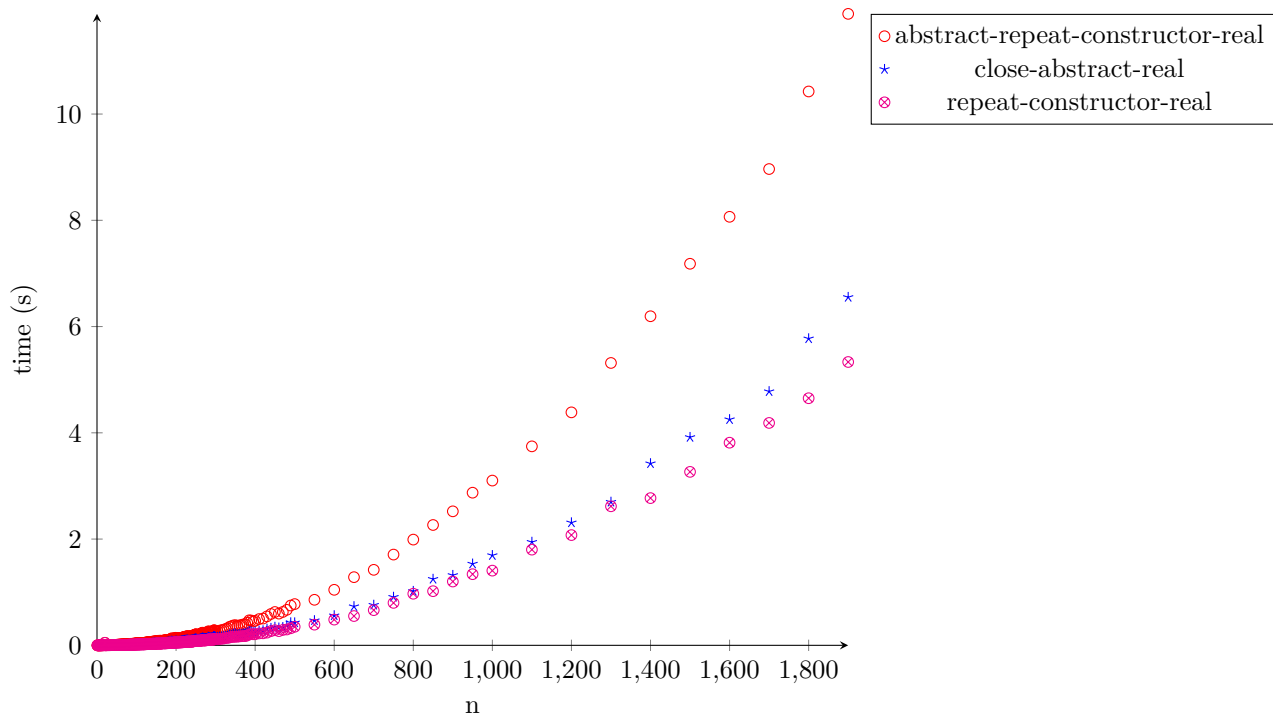
Figure 19: timing-conj-True-repeat-constructor
