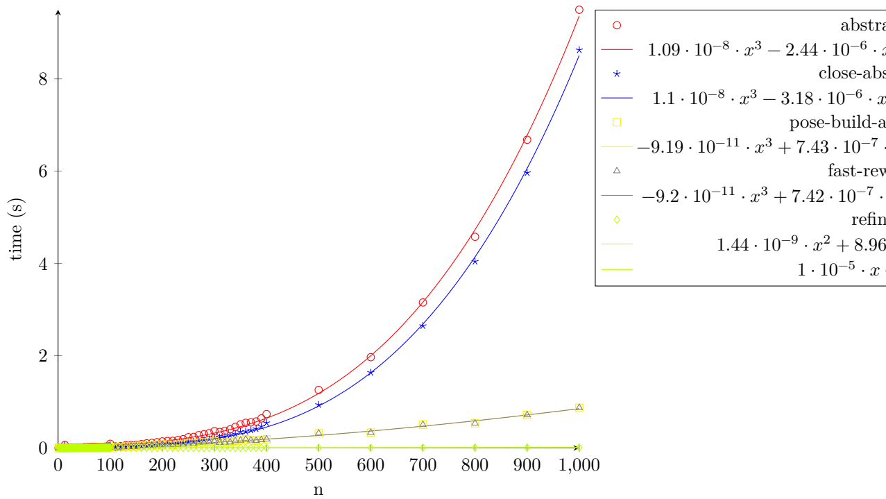
Figure 26: timing-rewrite-repeated-app-fast-rewrite
