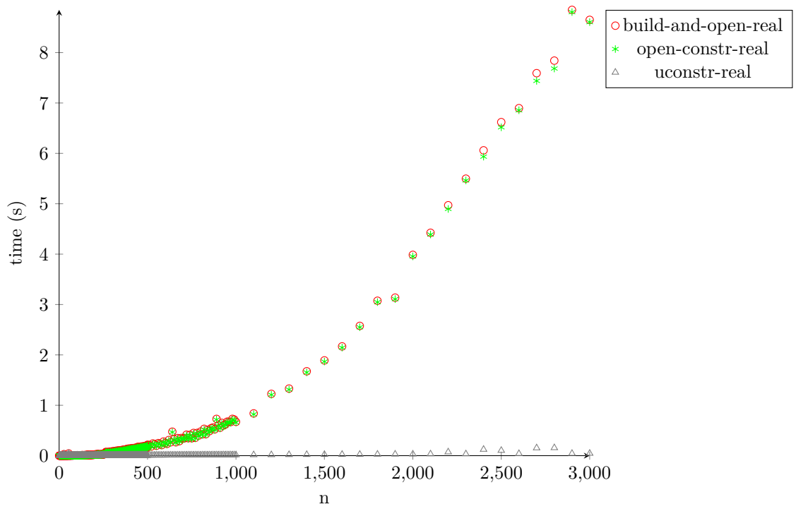
Figure 6: timing-open-constr-n-lambda-no-types-same-names
