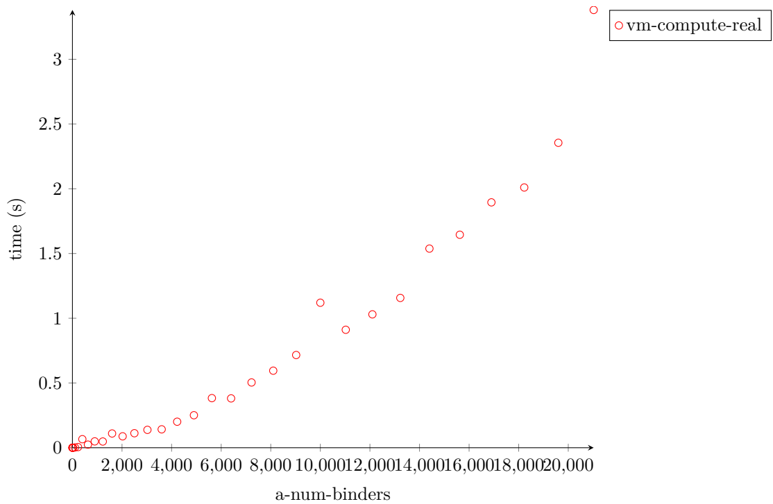
Figure 45: timing-quadratic-vm-PHOAS param-n 0
