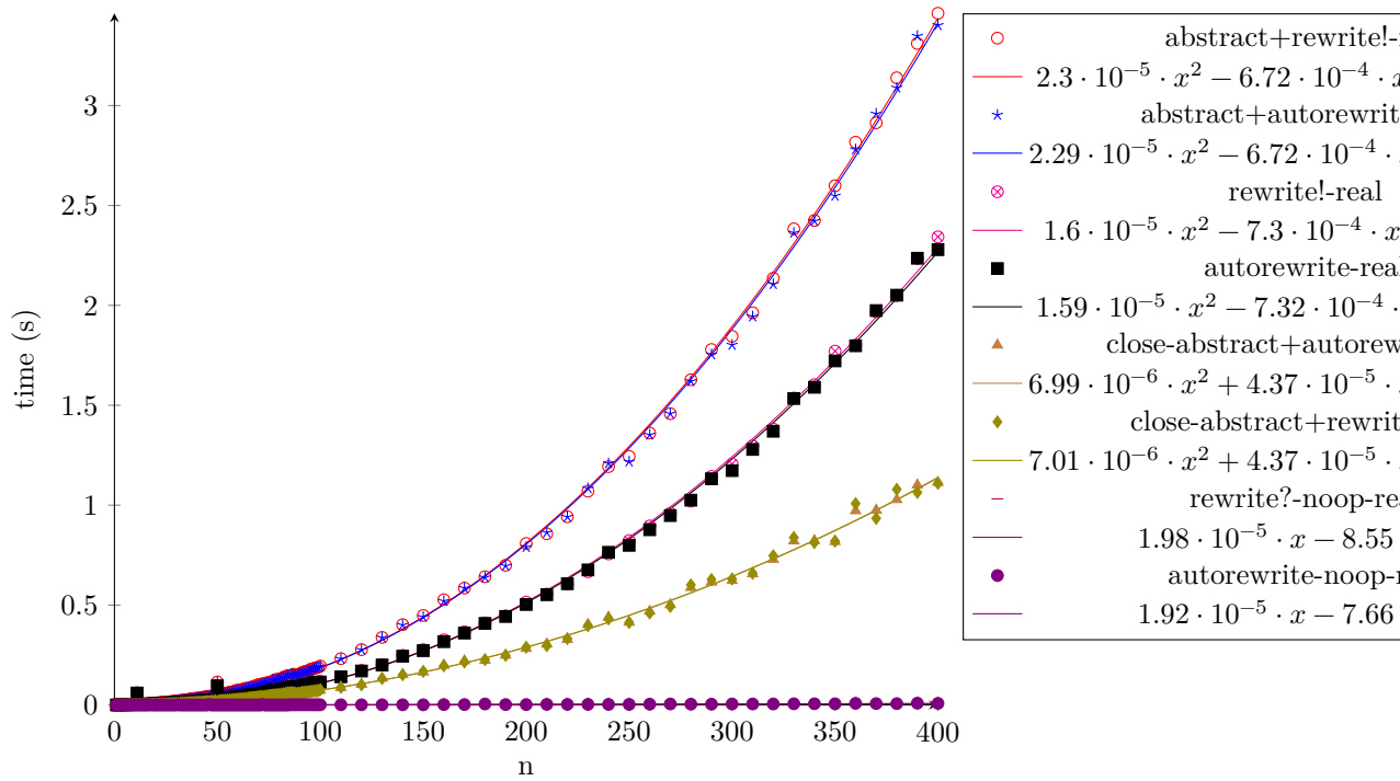
Figure 21: timing-rewrite-repeated-app-autorewrite
