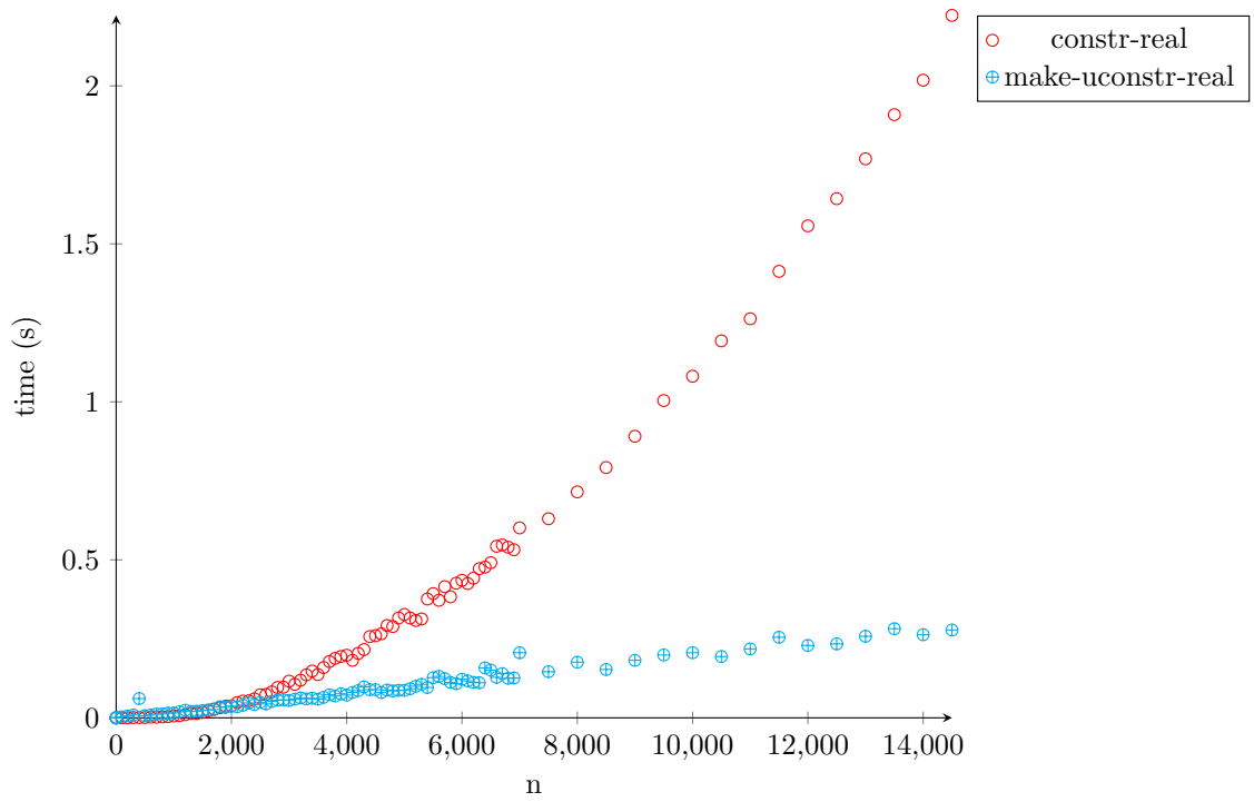
Figure 13: timing-fun-n-uconstr
