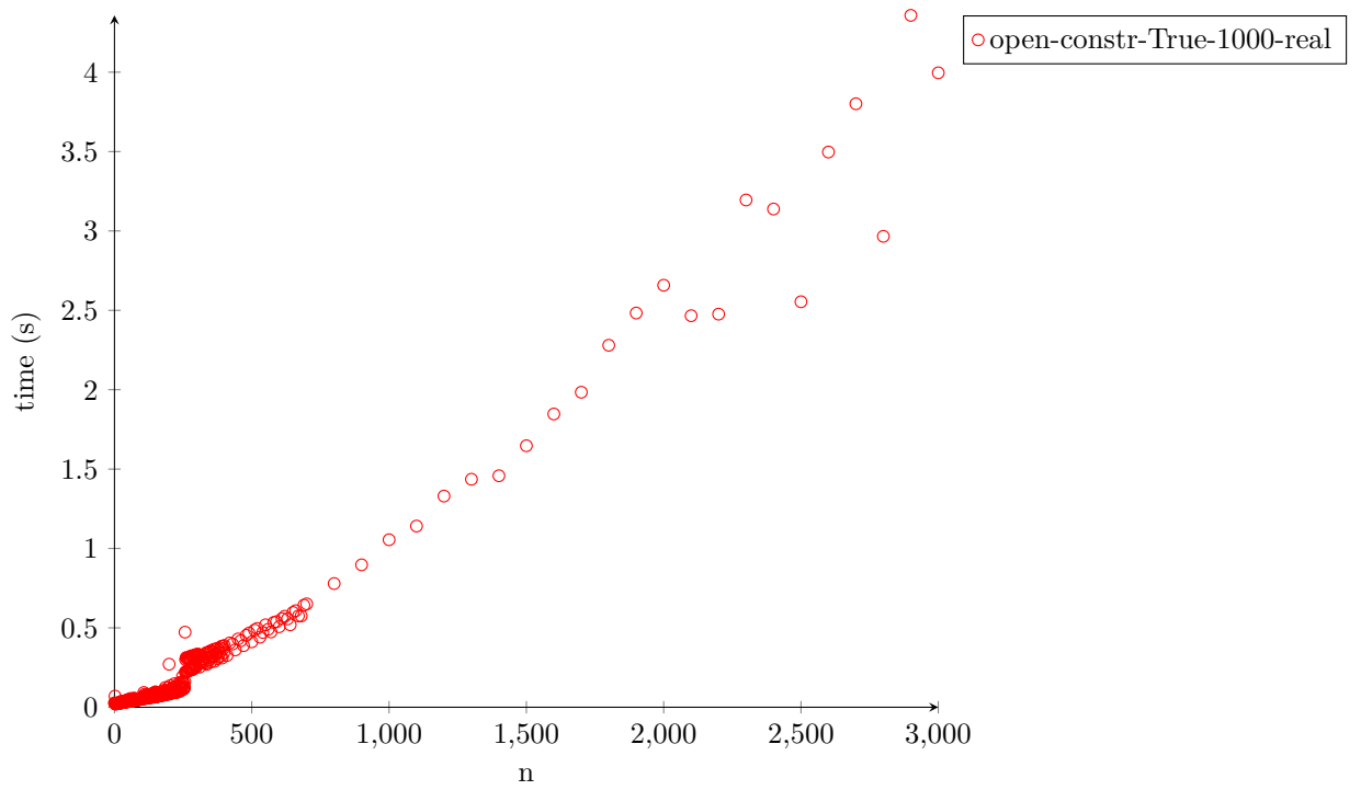
Figure 3: timing-do-n-open-constr-True
