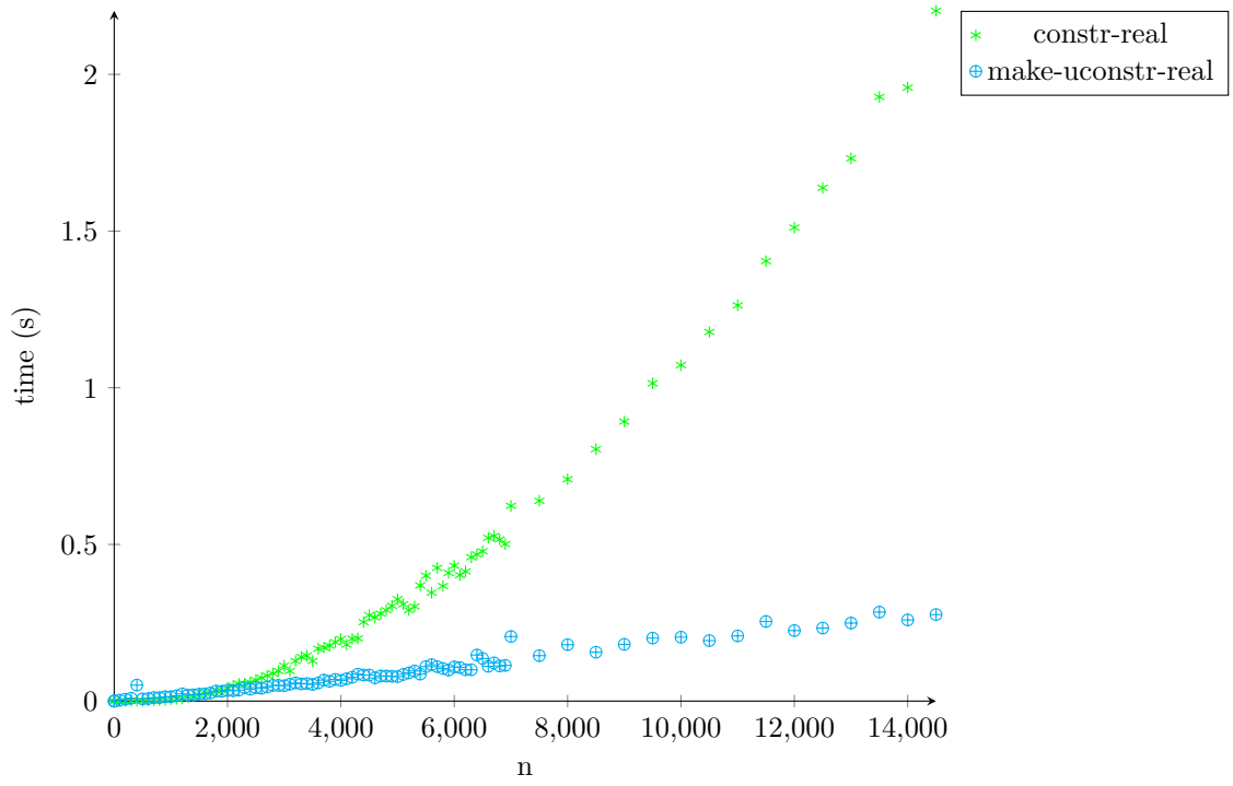
Figure 10: timing-let-n-uconstr
