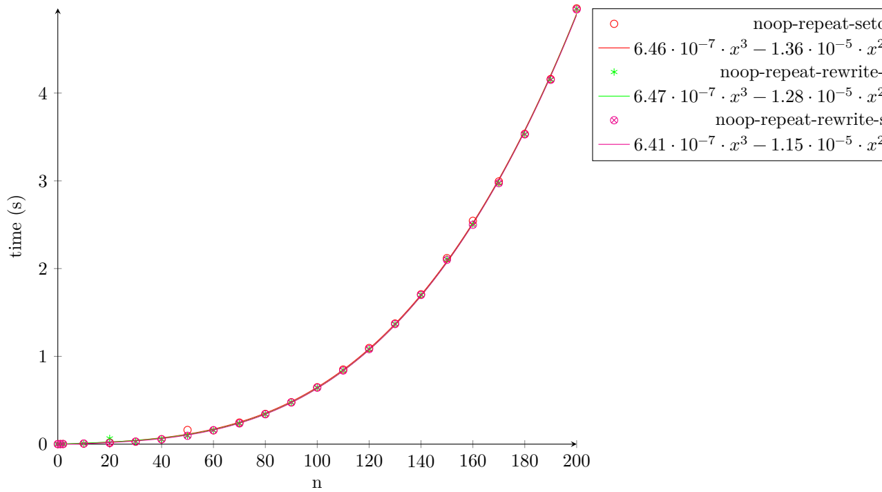
Figure 17: timing-repeat-setoid-rewrite-under-binders-noop
