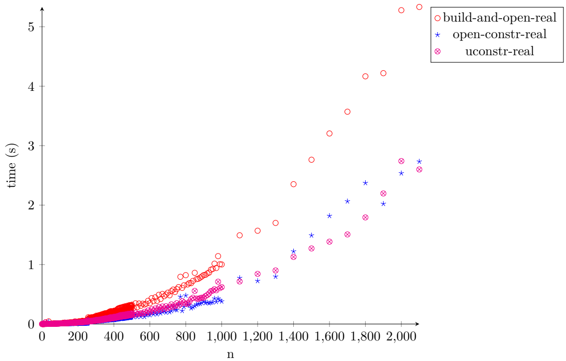
Figure 4: timing-open-constr-n-lambda-no-types-different-names
