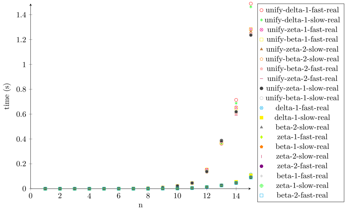
Figure 36: timing-one-step-reduction
