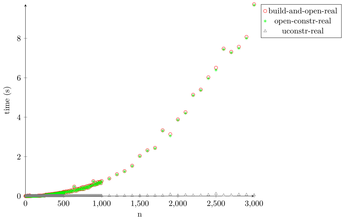
Figure 5: timing-open-constr-n-lambda-no-types-no-names
