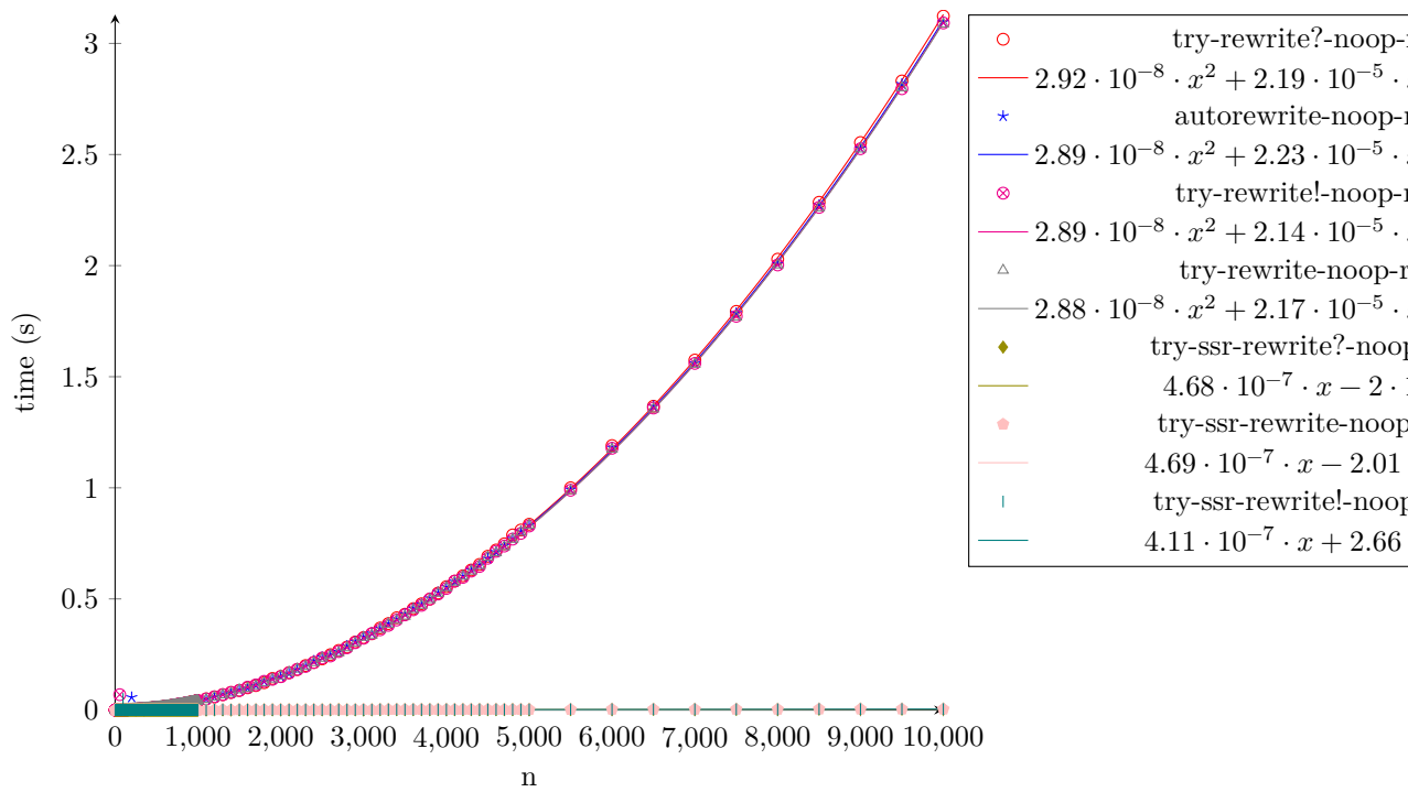
Figure 22: timing-rewrite-repeated-app-autorewrite-noop
