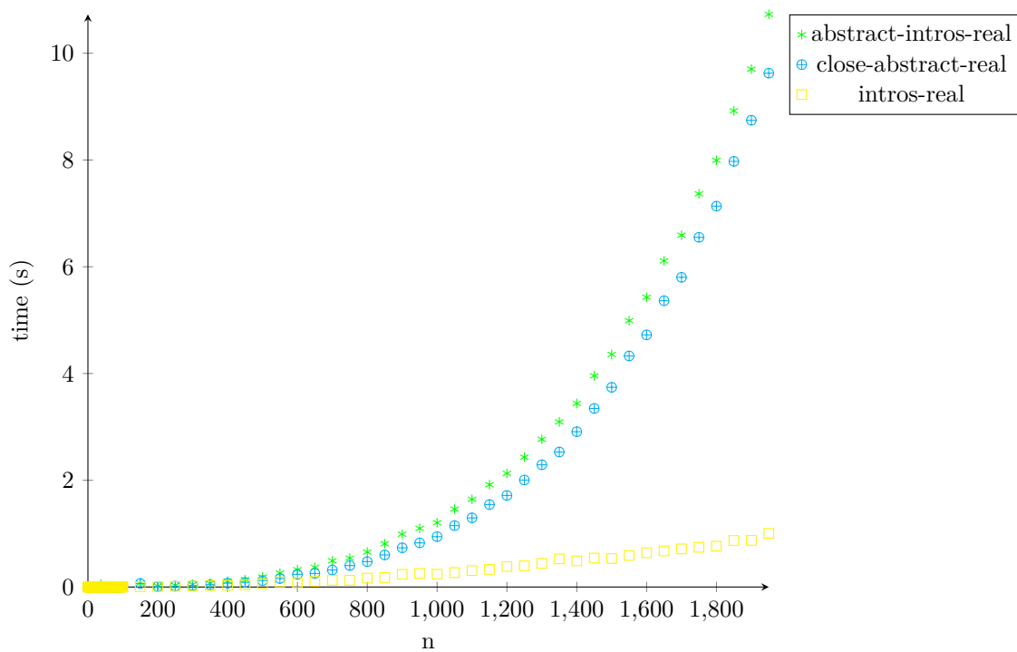
Figure 12: timing-intros-n-let
