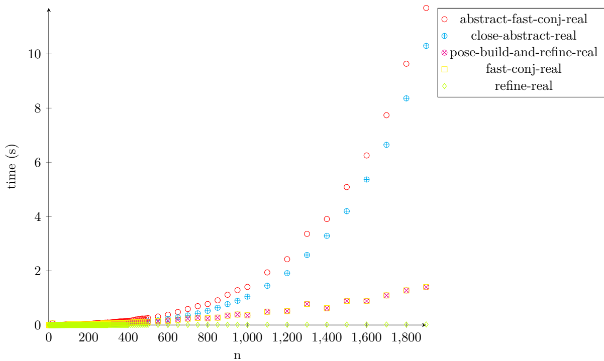
Figure 20: timing-conj-True-fast-conj
