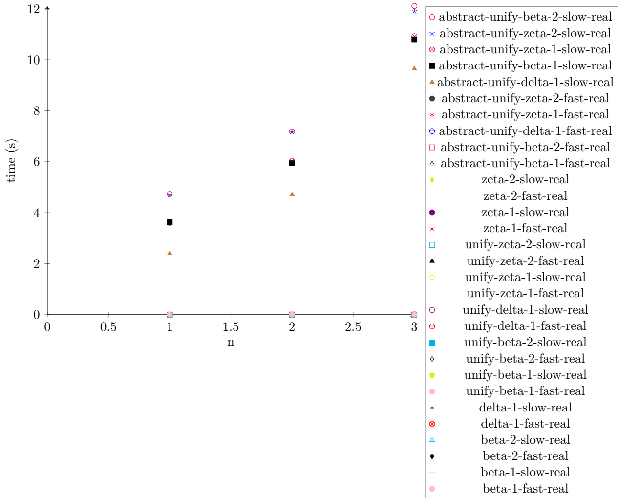
Figure 37: timing-one-step-reduction-with-abstract
