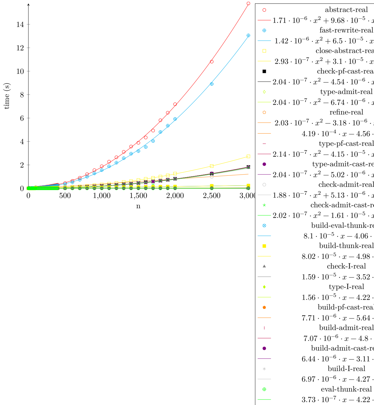
Figure 27: timing-rewrite-repeated-app-fast-rewrite-ltac2
