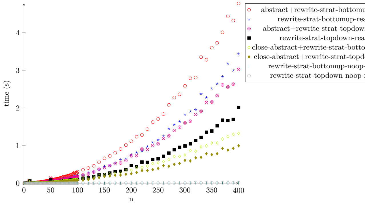
Figure 25: timing-rewrite-repeated-app-rewrite-strat
