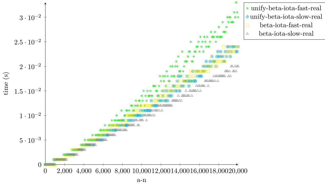
Figure 38: timing-iota-reduction-fact8 param-fact-n 8
