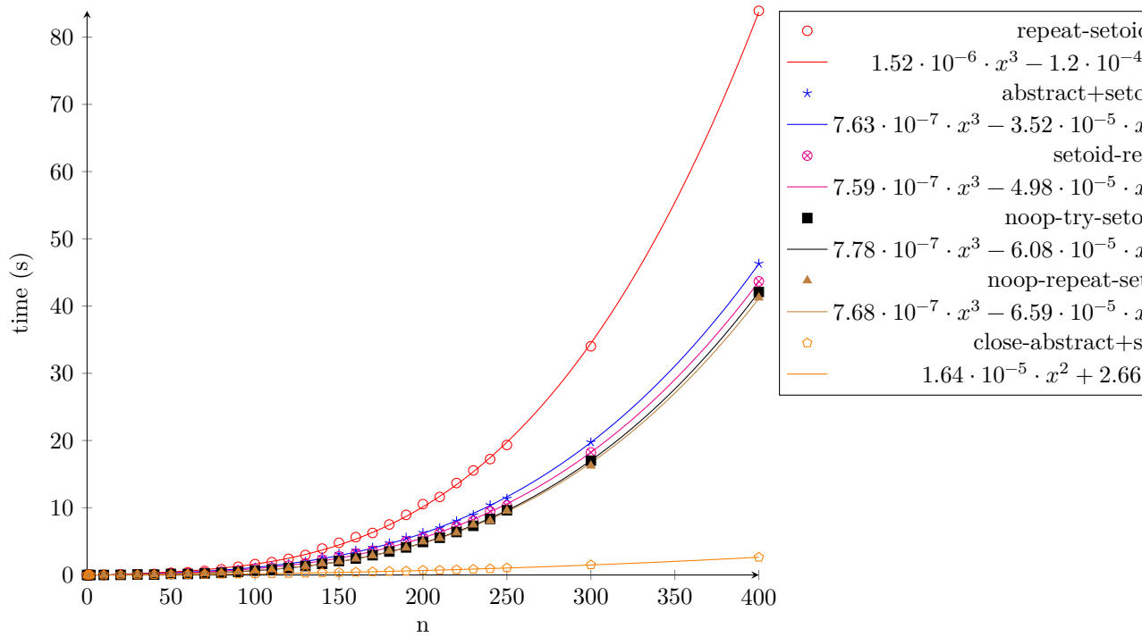
Figure 16: timing-repeat-setoid-rewrite-under-binders
