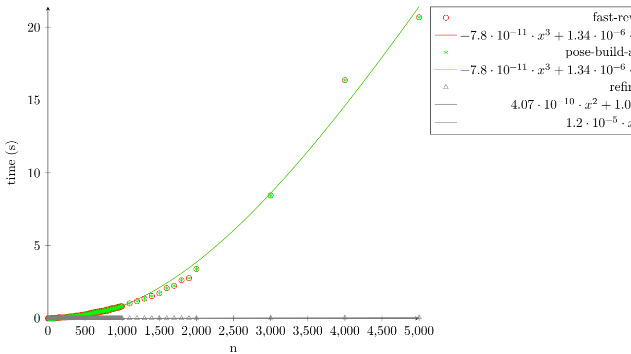
Figure 28: timing-rewrite-repeated-app-fast-rewrite-no-abstract
