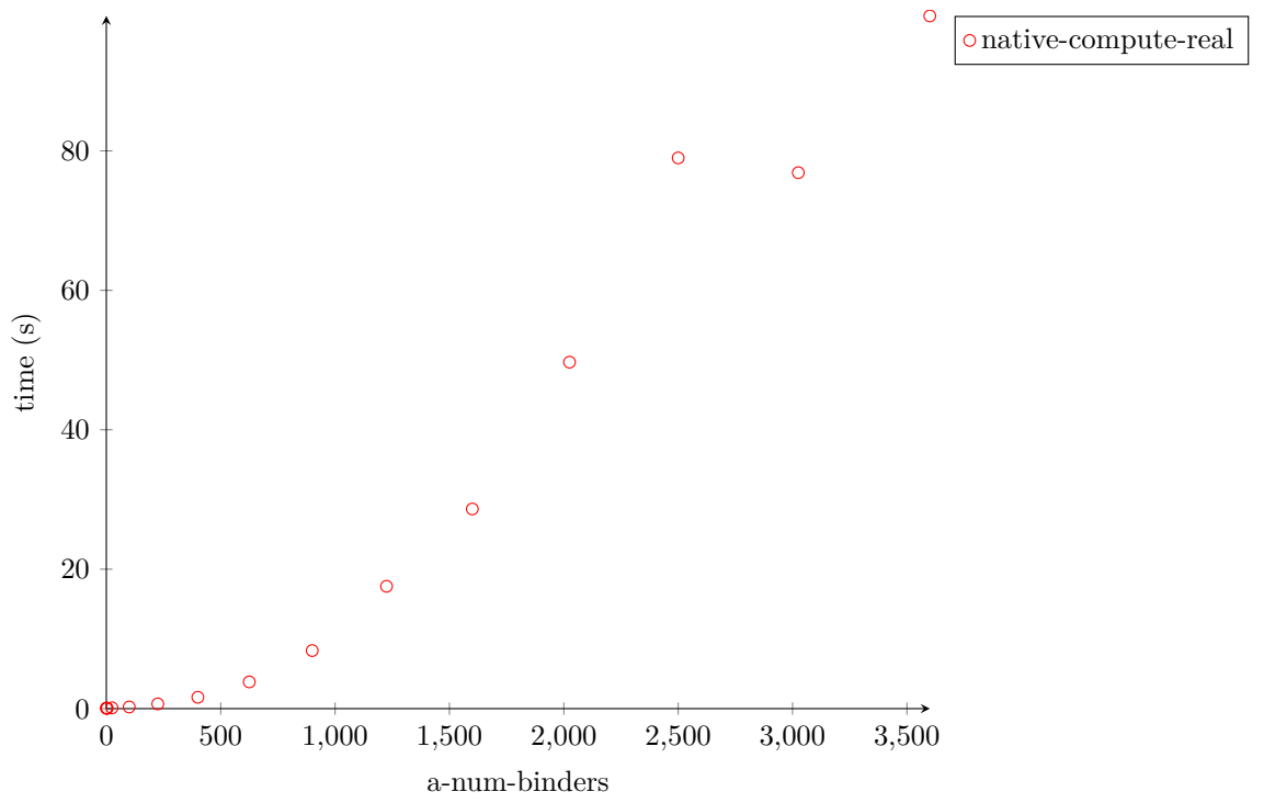
Figure 44: timing-quadratic-native-PHOAS param-n 0
